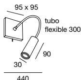
Ref 1695 1x 1,4w LED
