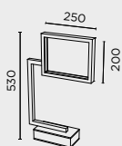
PS-191 LED 16W 2560lm 3000K
