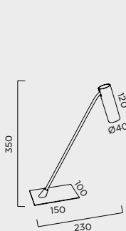
PS-44 1 x LED 5W 500lm 3000K
