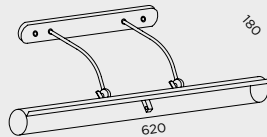
A-1006 4 x E-14 60W Max.
