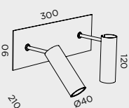
A-41 2 x LED 5W 500lm 3000K
