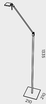
P-76 1 x LED 5W 500lm 3000K ON-OFF
