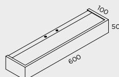
A-811/60 3 x R7s 78mm 80W Max. IP44
