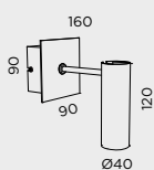
A-40 1 x LED 5W 500lm 3000K
