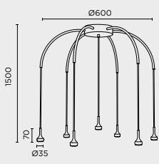
C-198/7 LED 21W 1365lm 3000K
