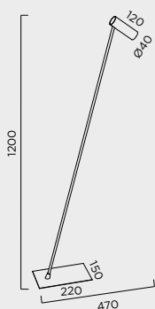
P-45 1 x LED 5W 500lm 3000K
